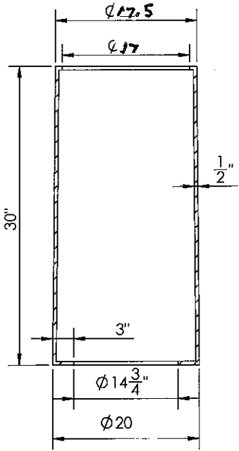
AA - 18-30HD5 HANDHOLE (1830HD5)
