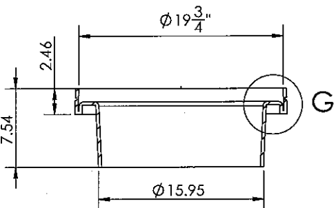
SECTION F-F SCALE 1 : 8
