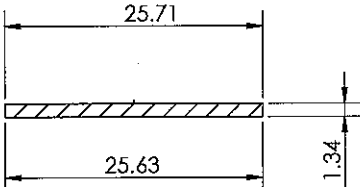
C - ELECTRIC COVER/LID (ESS19NC.)
