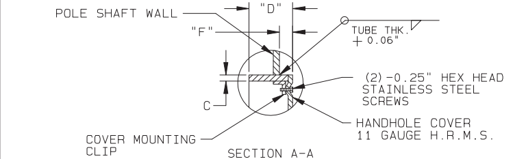
DETAIL 6 LOWER HANDHOLE
