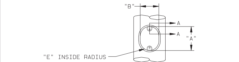
DETAIL 5 UPPER HANDHOLE
