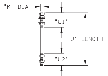
DETAIL 9 ANCHOR BOLT
