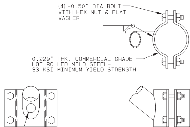
DETAIL 4 LUMINAIRE ARM ATTACHMENT (OPTIONAL)
