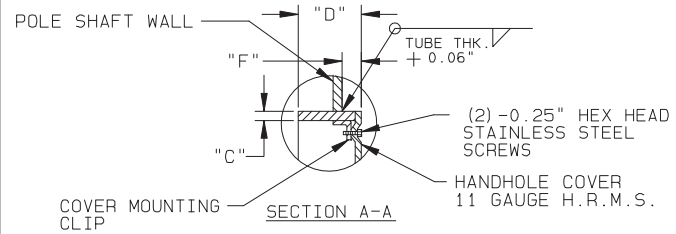
DETAIL 5 UPPER HANDHOLE
