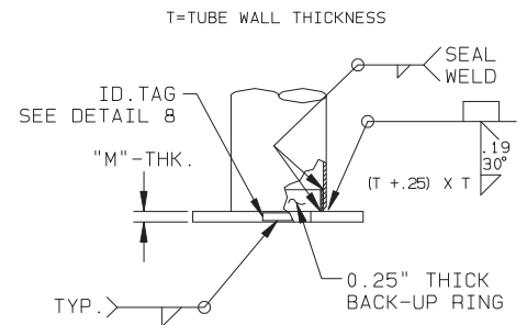
DETAIL 7 POLE BASE
