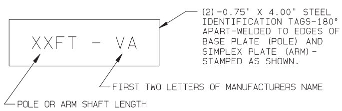
DETAIL 8 IDENTIFICATION TAG
