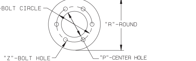
DETAIL 7 POLE BASE
