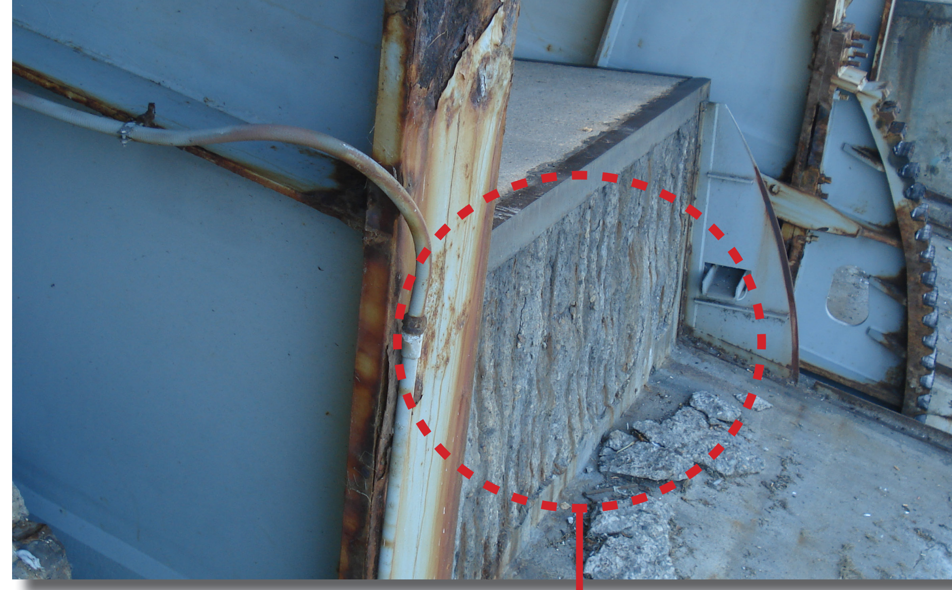
Heavy Concrete Deterioration with Exposed Rebar
