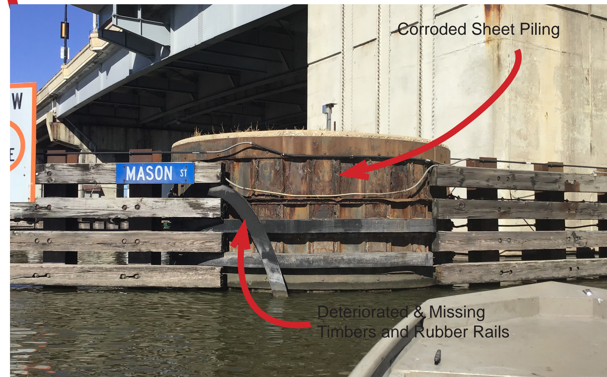
Repair Fender System
