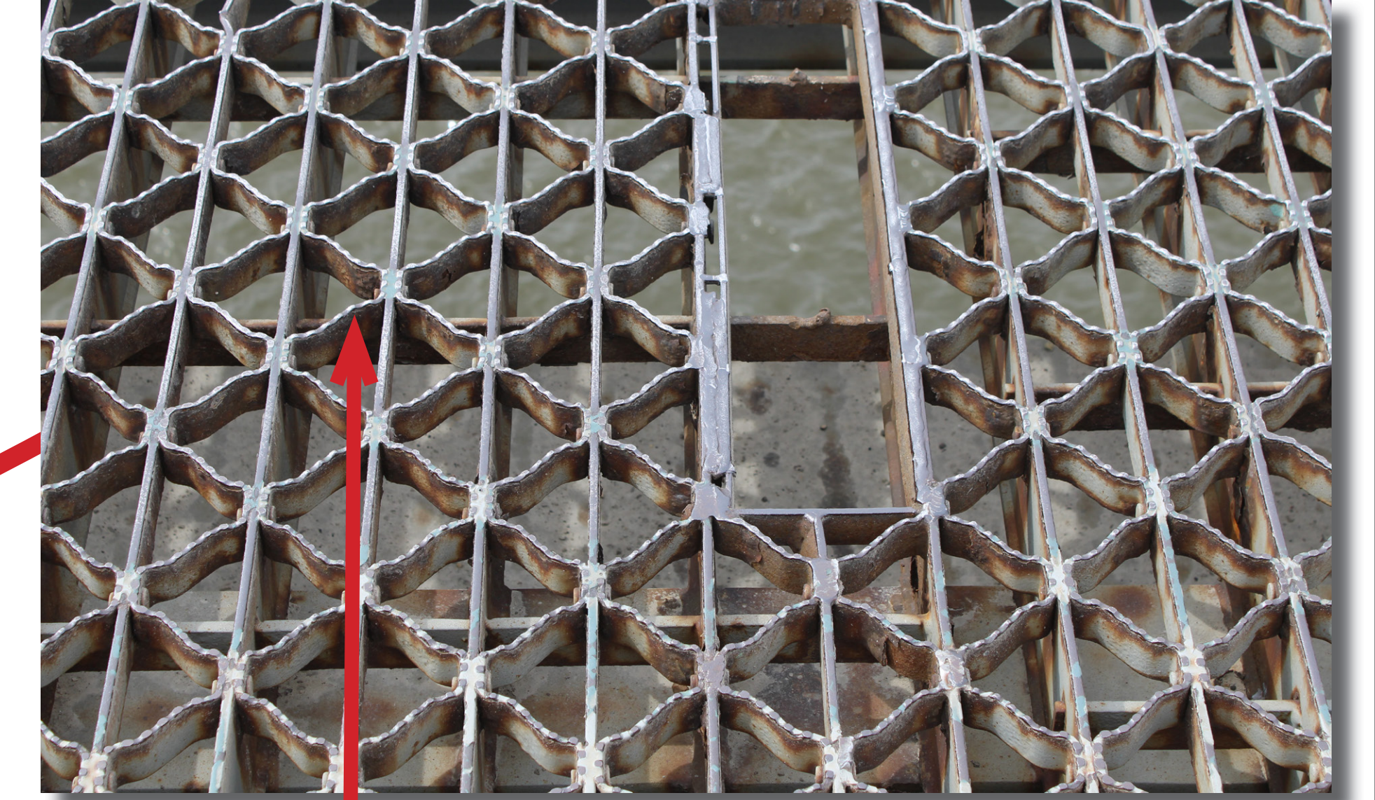
Numerous weld repairs on broken/missing bars. Grid Deck requires continuous repairs.
