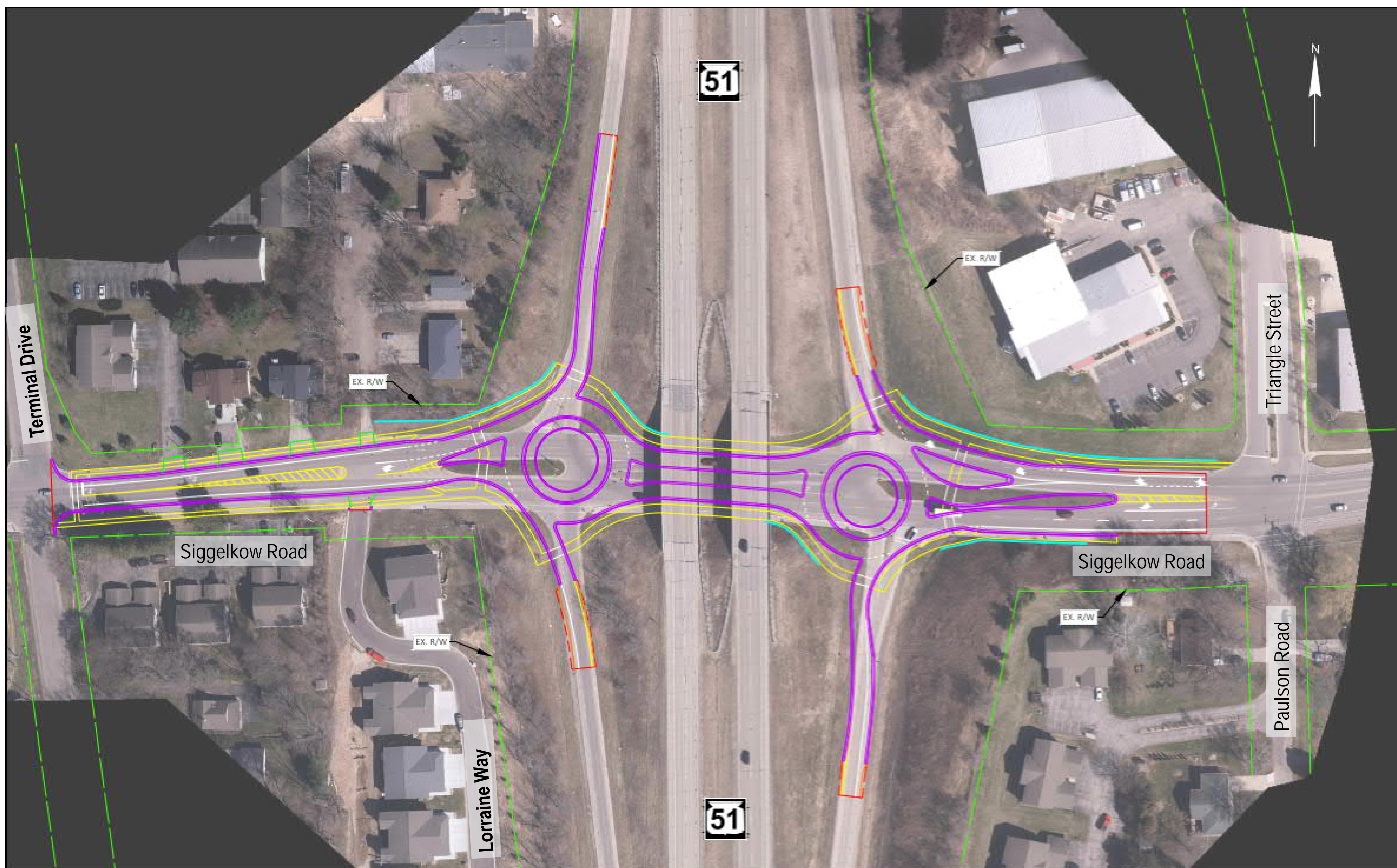
Roundabout option
