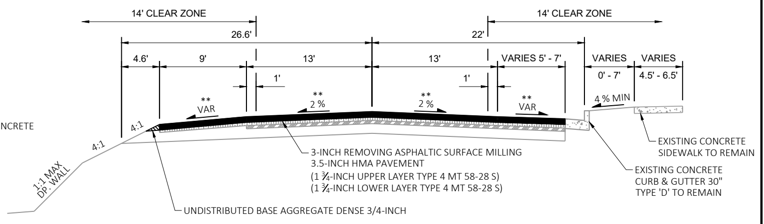
FINISHED FERRYVILLE TYPICAL SECTION
