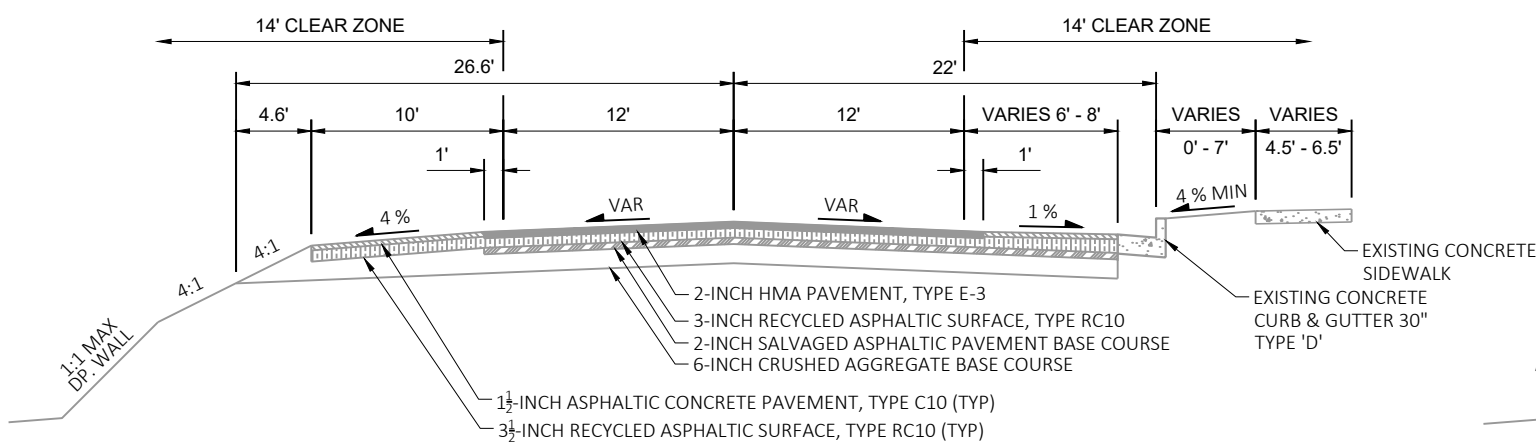
EXISTING FERRYVILLE TYPICAL SECTION
