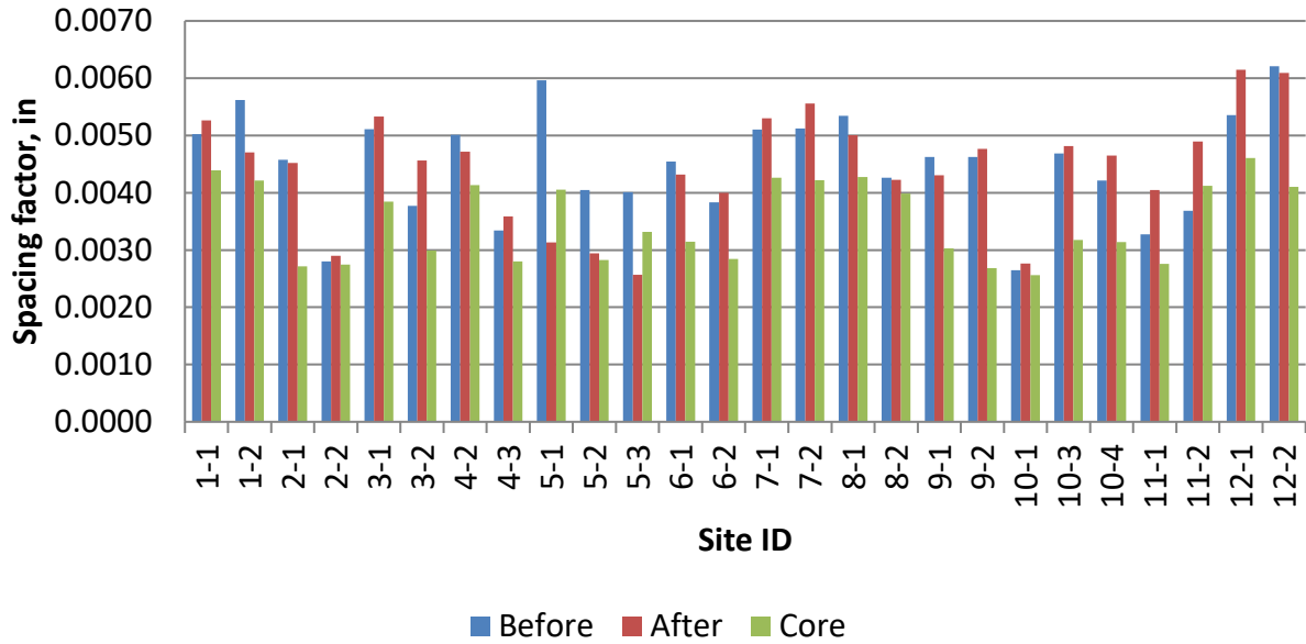
Figure 33. Spacing factor: cylinders vs drilled cores
