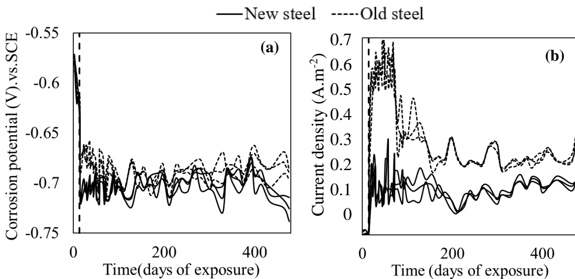
Figure 4.13. (a) Corrosion potential values and (b) corrosion current densities of new and old steels in water. Vertical dash line represents the data of chloride addition.
