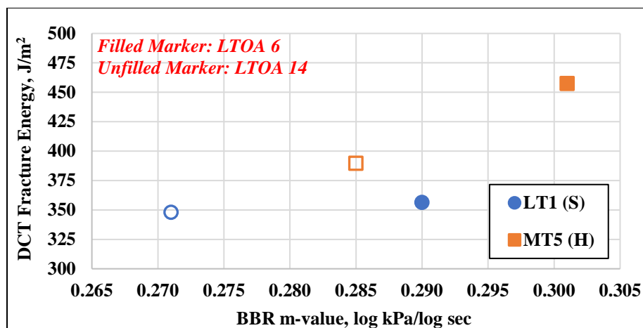
Figure 31. Average DCT Fracture Energy versus BBR m-value for Control Plant-Produced Mixtures at Different Aging Levels.
