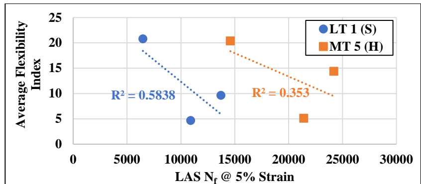
Figure 27. Average FI versus LAS N_f @ 5% Strain at Different Aging Levels.
