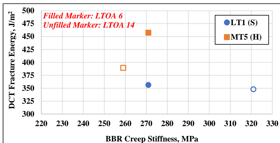
Figure 32. Average DCT Fracture Energy versus BBR Creep Stiffness for Control Plant-Produced Mixtures at Different Aging Levels.
