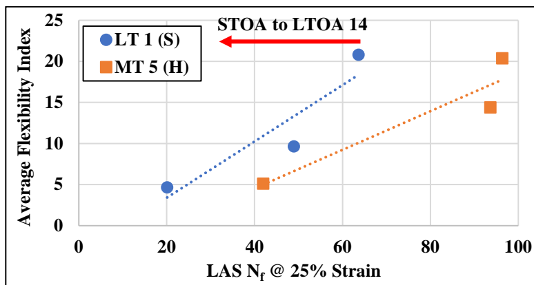
Figure 29. Average FI versus LAS N_f @ 25% Strain at Different Aging Levels.
