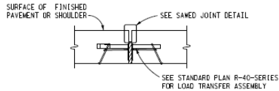
Figure 60. Transverse expansion joints (Michigan DOT 2020a).
