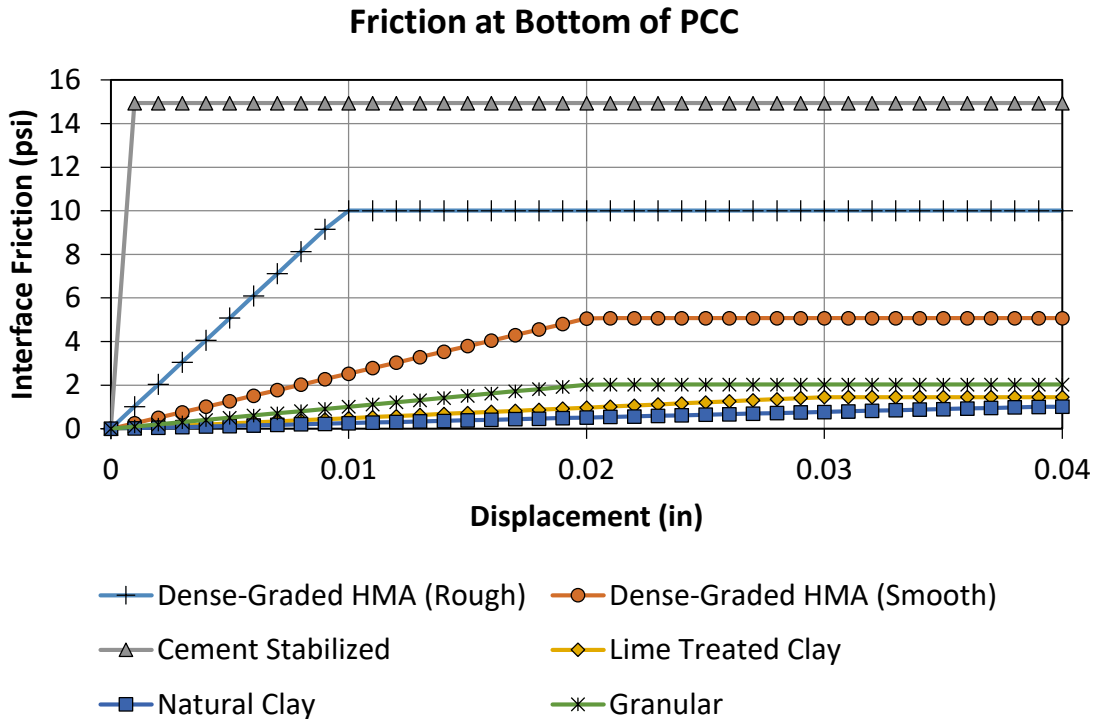
Figure 30. Friction at PCC slab and base interface.
