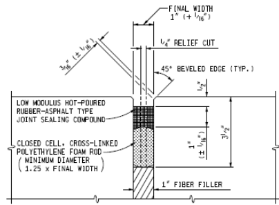
SAWED JOINT DETAIL SAWED JOINT SEALED WITH LOW MODULUS HOT-POURED RUBBER-ASPHALT TYPE JOINT SEALING COMPOUND.
