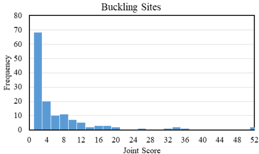
Figure 25. Joint scores of buckling sites.
