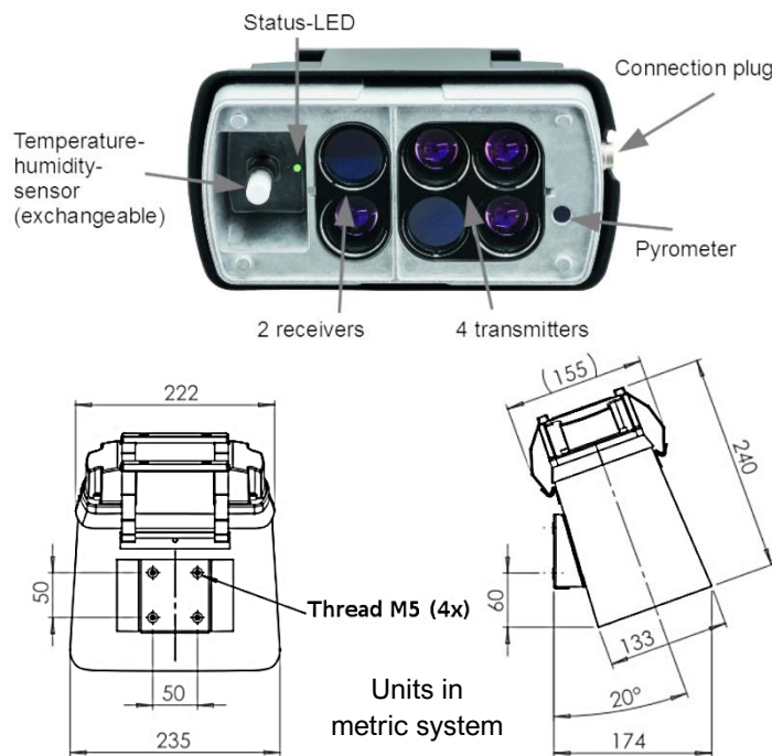
Figure 2. MARWIS friction data collection device (Lufft 2019)
