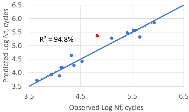
Figure 22. Observed and Predicted Fatigue Life Using Log G* and CTindex at 20/26°C as Predictors, with 26°C Data Point Omitted from Calculation of R 2 .
