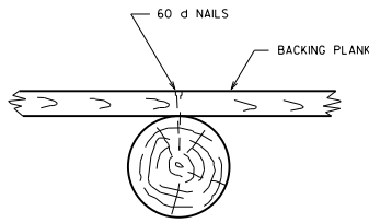
TIMBER PILING
