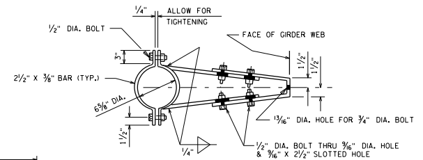
BRACKET DETAIL
