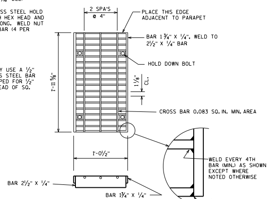
GRATE DETAIL
