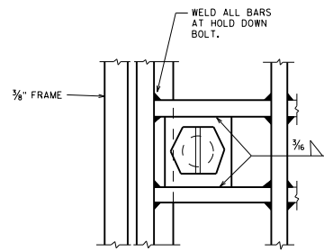
PART PLAN
