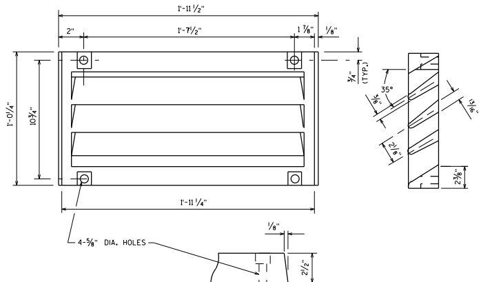
GRATE CASTING DETAIL
