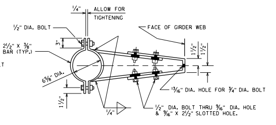
BRACKET DETAIL
