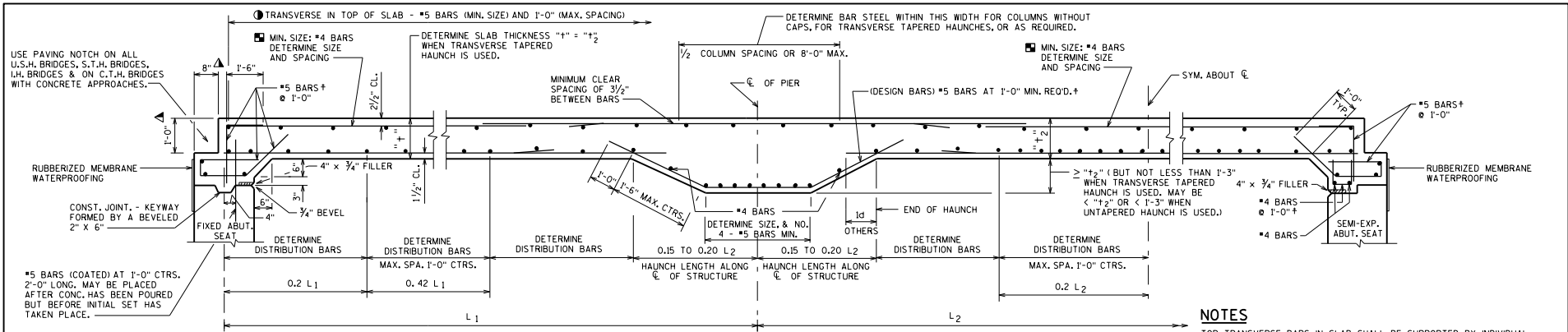
LONGITUDINAL SECTION † BARS PLACED PARALLEL TO \bar{C} SPACING PERPENDICULAR TO \bar{C} .
