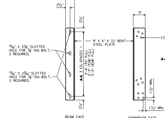
DIAPHRAGM SUPPORT
