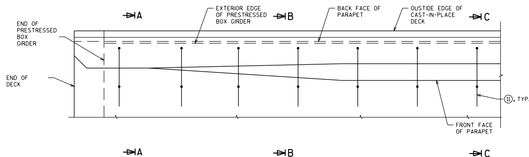
PLAN SHOWING REINFORCEMENT CAST INTO PRESTRESSED BOX GIRDER PARAPET AND DECK ARE SHOWN FOR CLARITY
