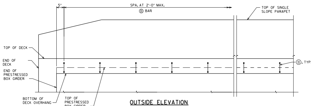
OUTSIDE ELEVATION SHOWING REINFORCEMENT CAST INTO PRESTRESSED BOX GIRDER PARAPET AND DECK ARE SHOWN FOR CLARITY
