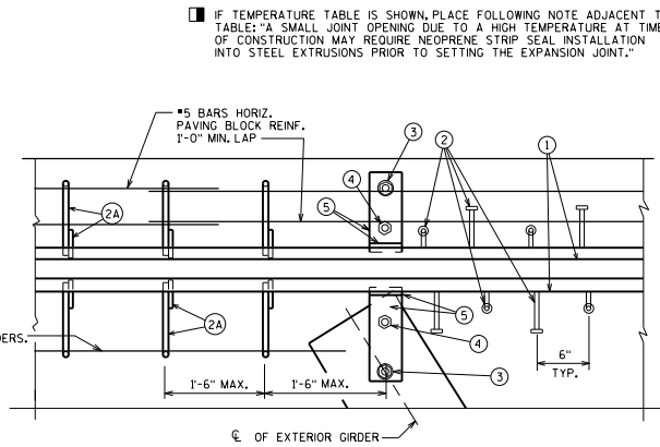
PART PLAN
