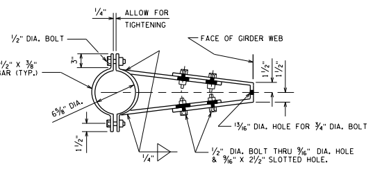
BRACKET DETAIL
