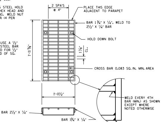
GRATE DETAIL
