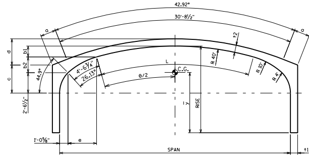
28'-0" TO 42'-0" SPANS
