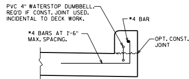
CURB DETAIL
