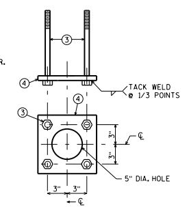
ANCHORAGE DETAIL
