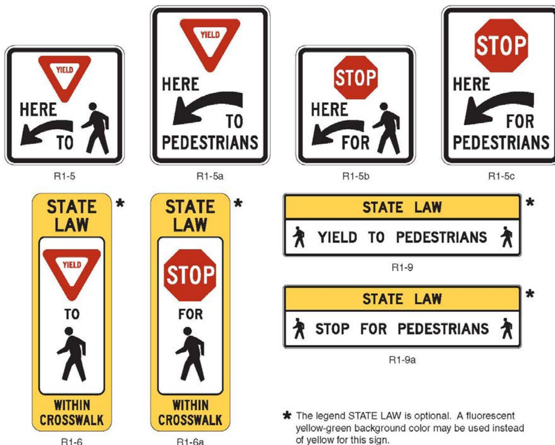
Figure 2B-2. Unsignalized Pedestrian Crosswalk Signs
