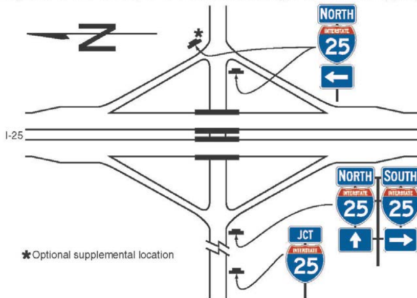
Figure 2D-12. Example of Minor Interchange Crossroad Signing
