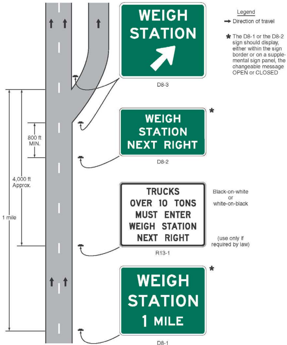
Figure 2D-17. Example of Weigh Station Signing
