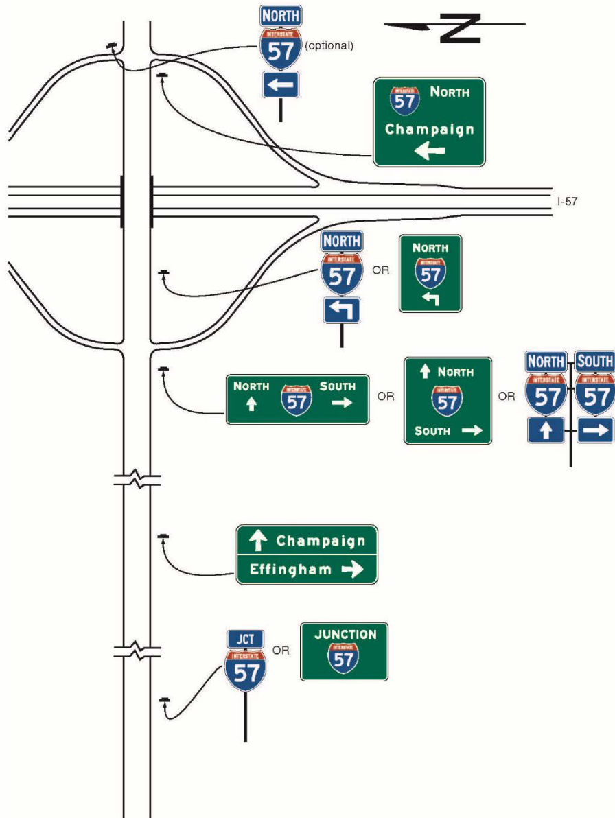
Figure 2D-12. Example of Minor Interchange Crossroad Signing
