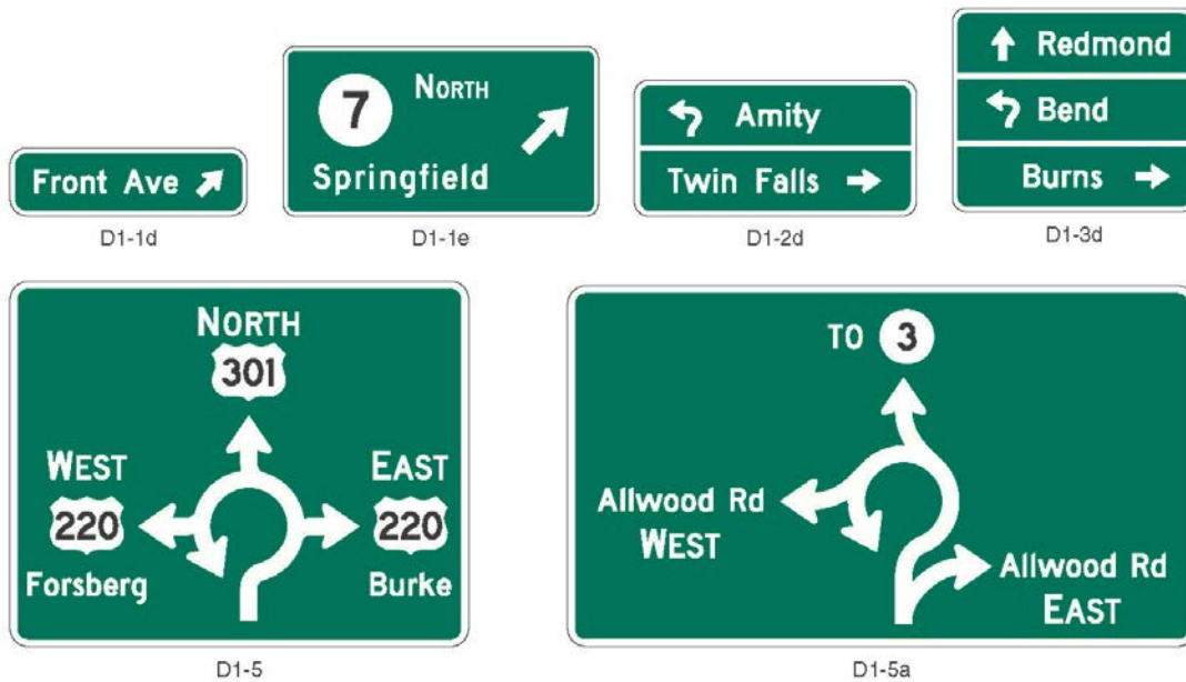
Figure 2D-8. Destination Signs for Roundabouts
