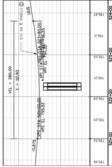
STH 54 PROFILE
