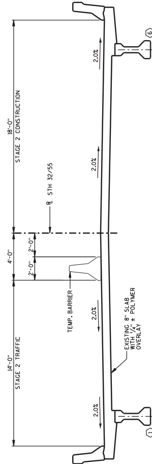
CROSS SECTION THRU BRIDGE - STAGE 2 (LOOKING NORTH)
