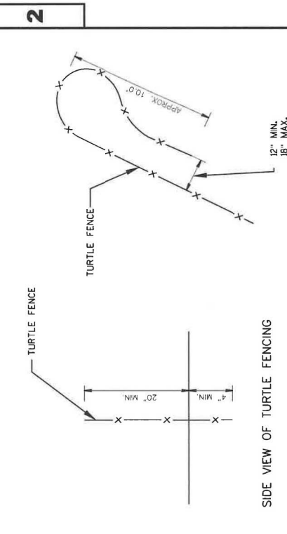
TURTLE FENCING WILL BE PAID UNDER STANDARD BID ITEM #628.1504, SILT FENCE.
