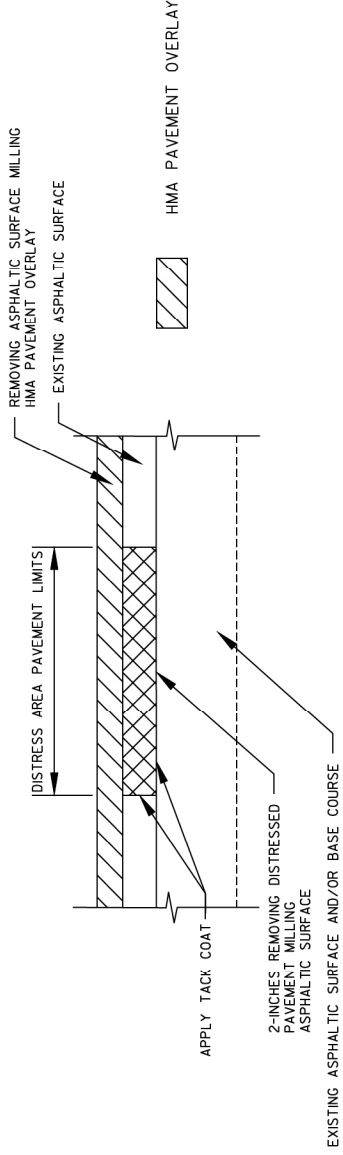
REMOVING DISTRESS PAVEMENT MILLING SECTION A-A
